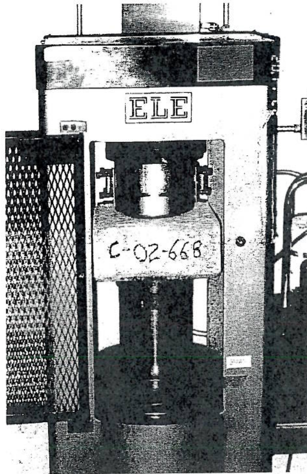
Photograph 5 – Testing configuration in compressive strength machine.
