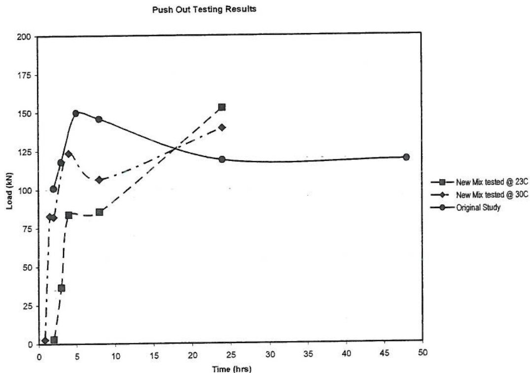
Figure 3 – Results of the Pushout Testing
