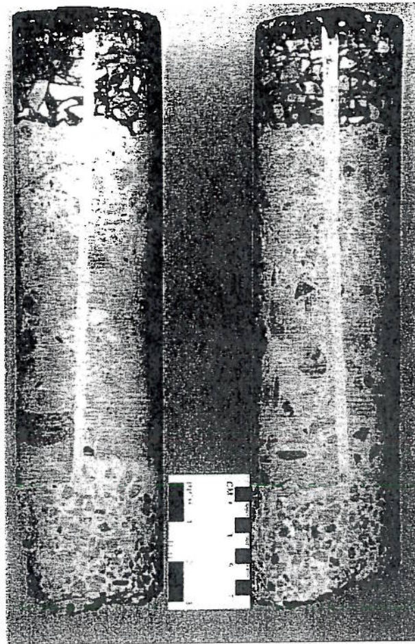
Photo 5 – View of satellite cores taken one month after installation in 1995.
