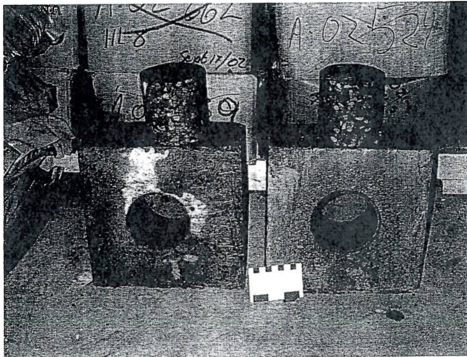
Photograph 1 – Test slabs with samples removed.
