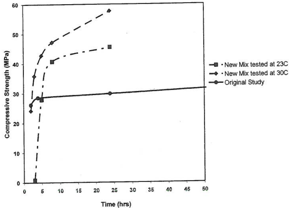
Figure 1 – Cube Strengths of the Utilibond™
