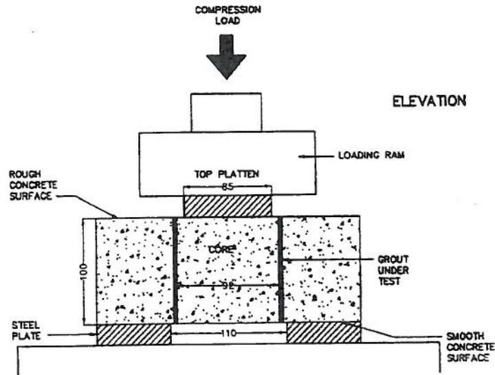
Figure 2 – Test set-up for simulated loading.
