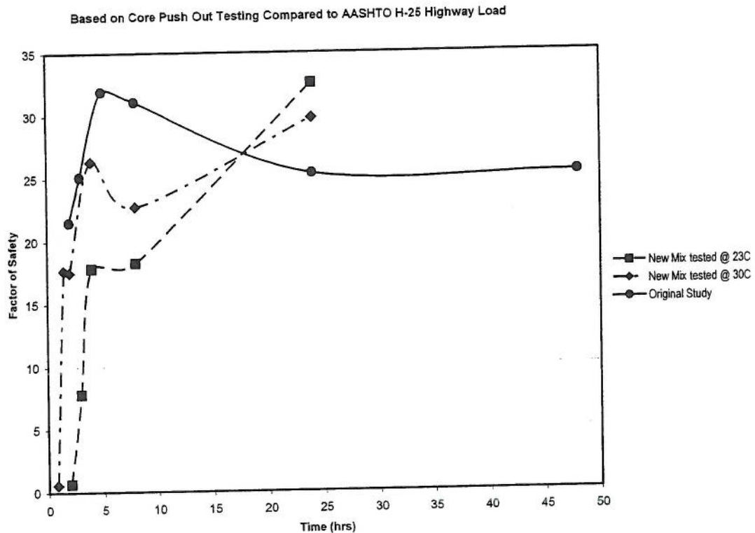
Figure 4 – Factor of Safety vs. AASHTO H-25 Loading
