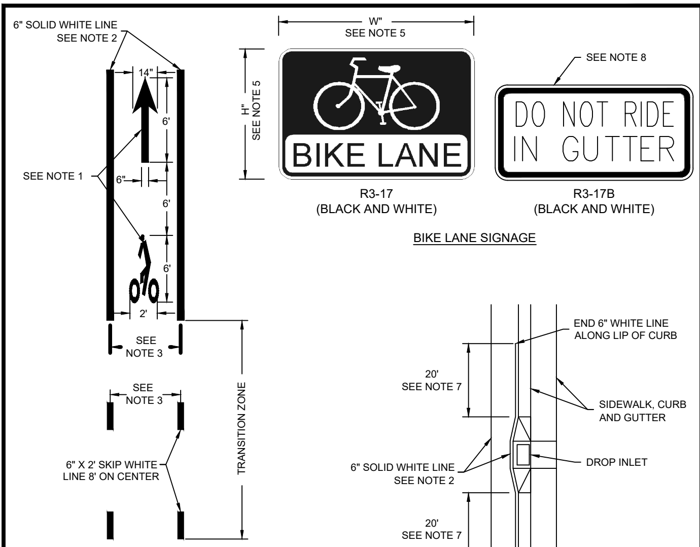
BIKE LANE DELINEATION AND LEGEND
